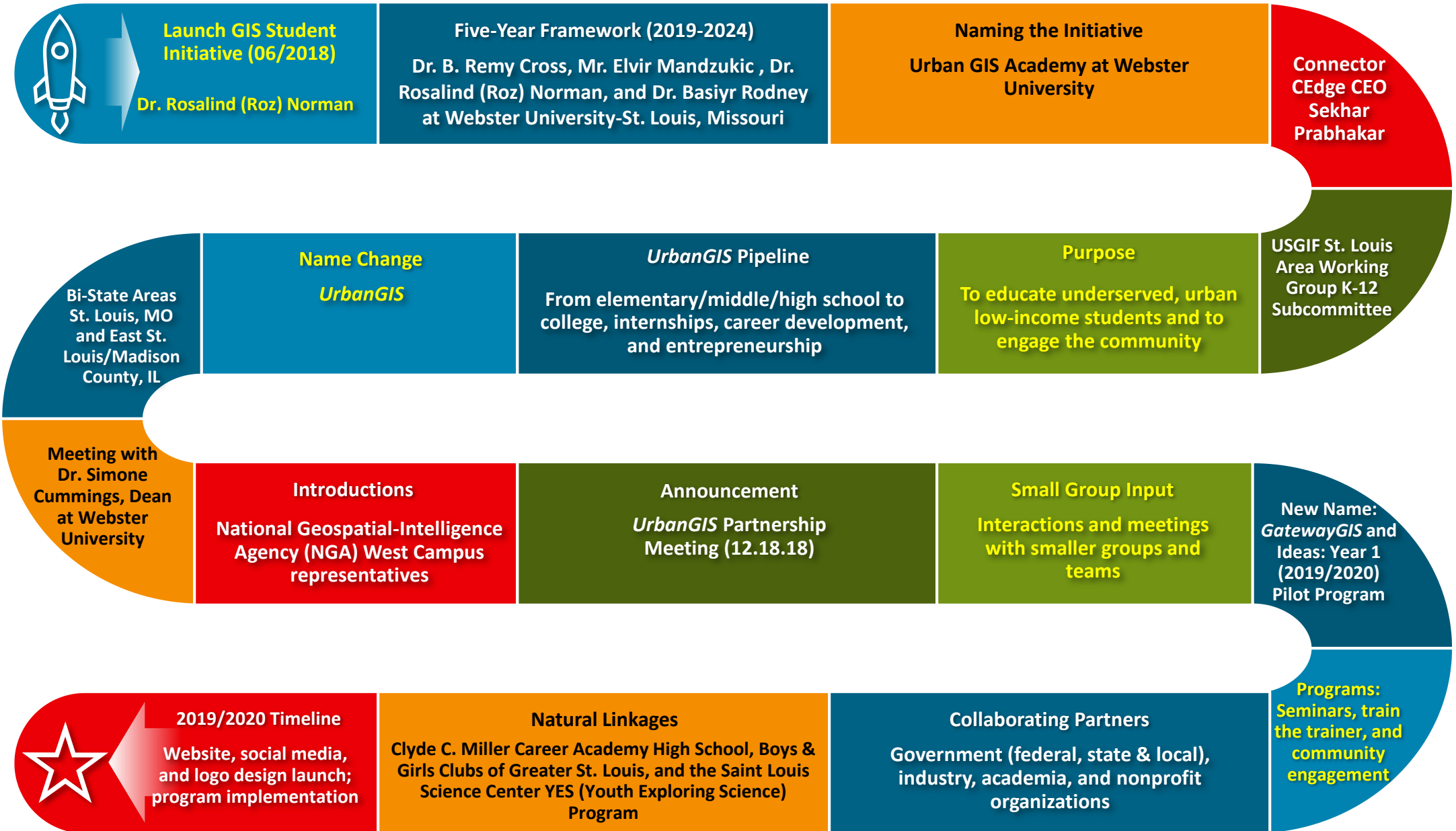
GatewayGIS Flowchart (03.29.19)
